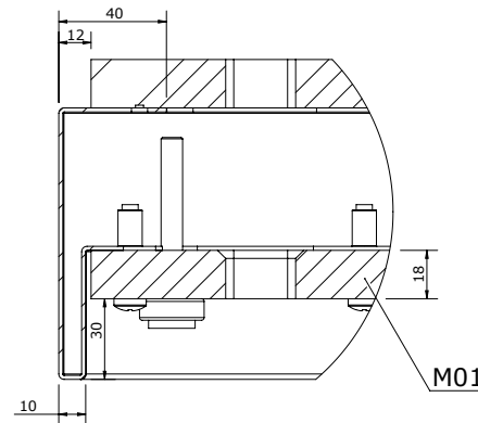
Detail B Scale 1 : 2
